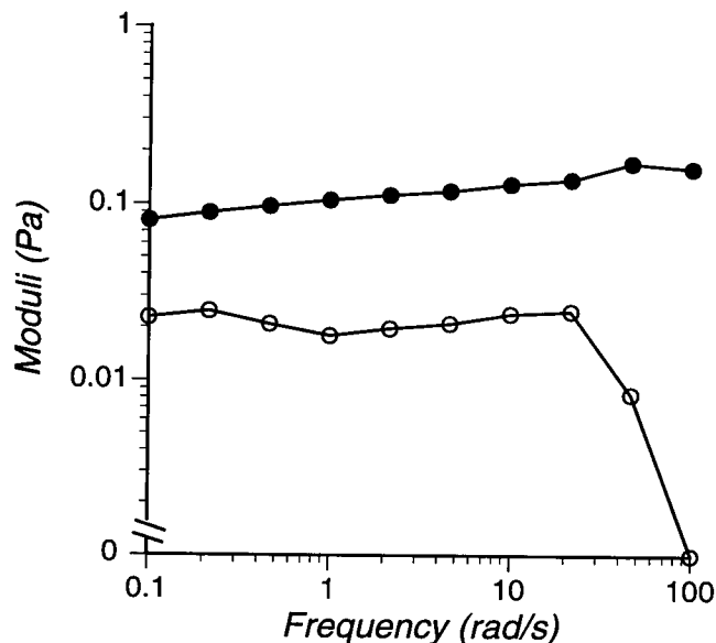
FIGURE 7 Oscillatory shear measurement on 0.4 mg/ml collagen gel with a frequency scan from 0.1 to 100 rad/s and 2% strain, G' ( \circ ) and G'' ( \bullet ). Gel breakdown appears to begin at frequencies higher than \sim 20 rad/s, as shown in the drop of G'' .
